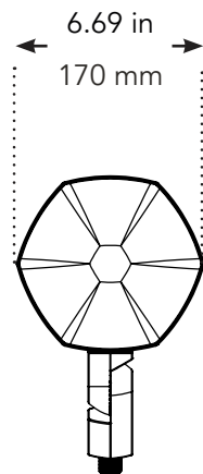
(A) Speaker Front View with Grille
