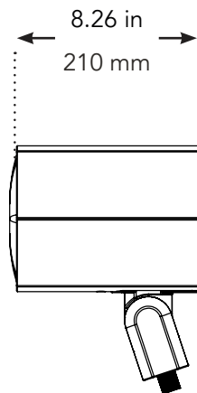
(B) Speaker Side Profile
